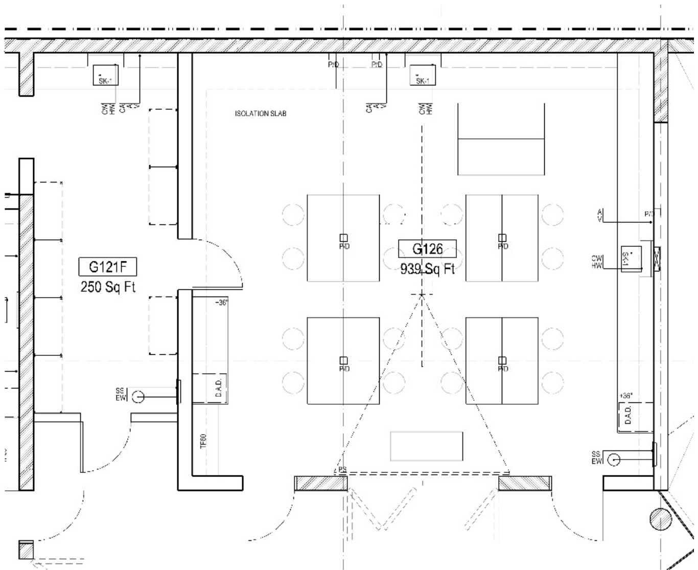
Figure 5: Detail of Upper-Division Physics Laboratory at the G1 level of the Center for Science and Innovation.
