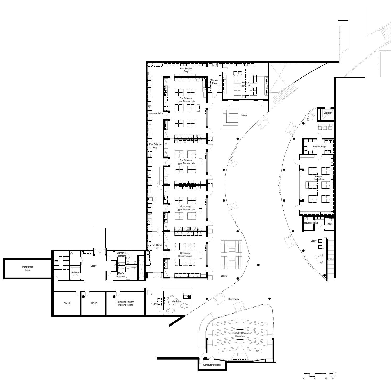
Figure 3: Floorplan of level G1 of the planned Center for Science and Innovation.
